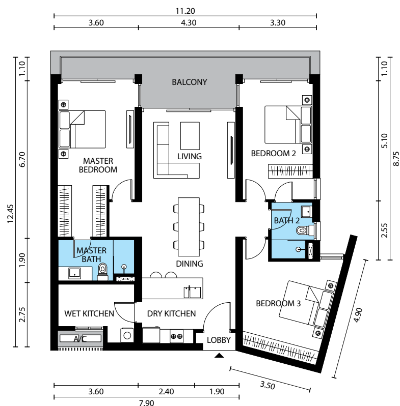
Floor Plan of units in level 13 & 23 (For others, the dimensions are slightly larger)
