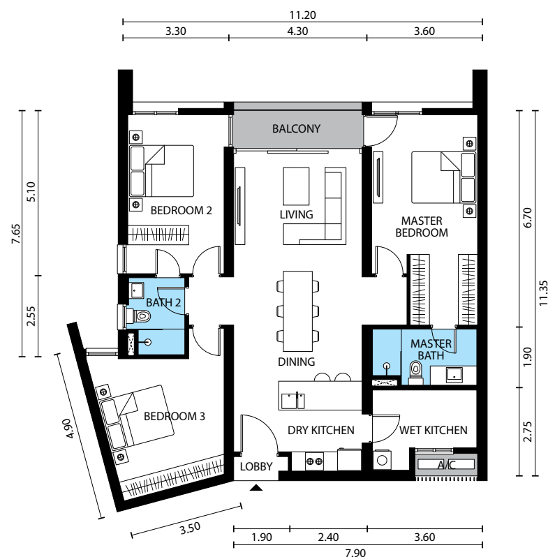
Floor Plan of units in level 17 & 18 (For others, the dimensions are slightly larger)
