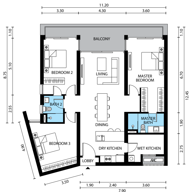
Floor Plan of units in level 15 & 19 (For others, the dimensions are slightly larger)
