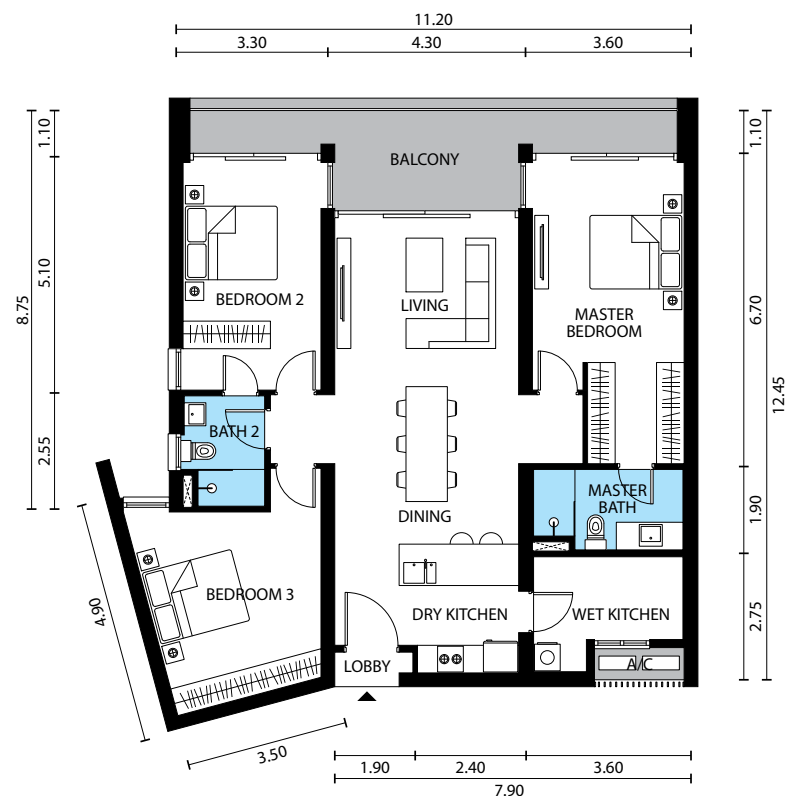
Floor Plan of units in level 3a, 16 & 20 (For others, the dimensions are slightly larger)
