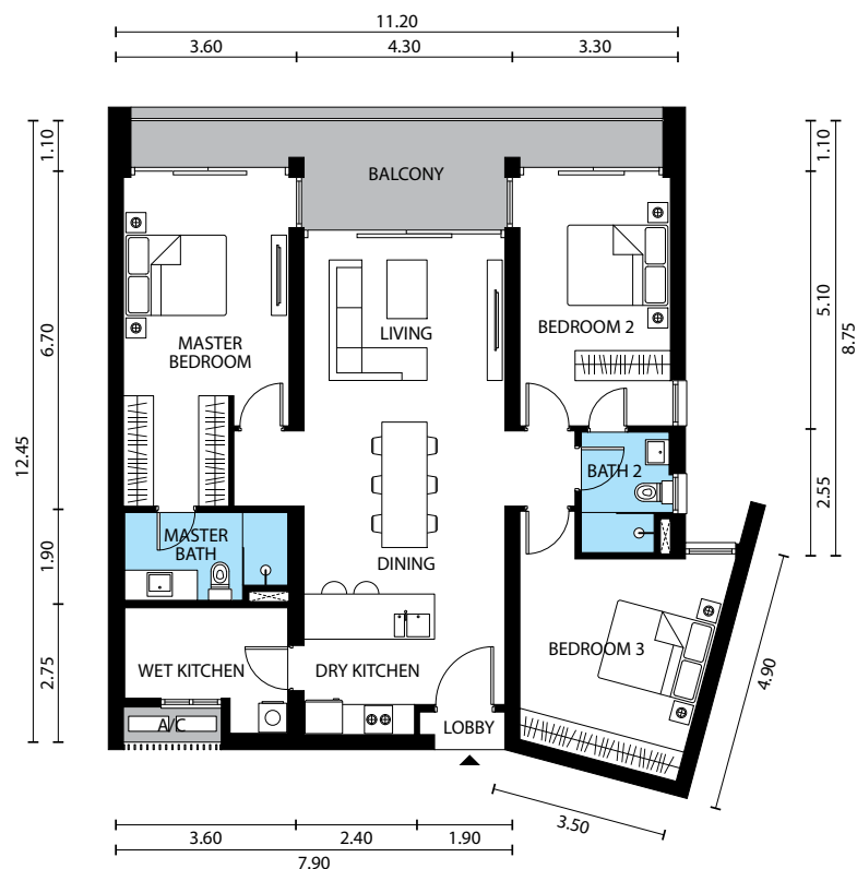
Floor Plan of units in level 3a, 13a & 23a (For others, the dimensions are slightly larger)
