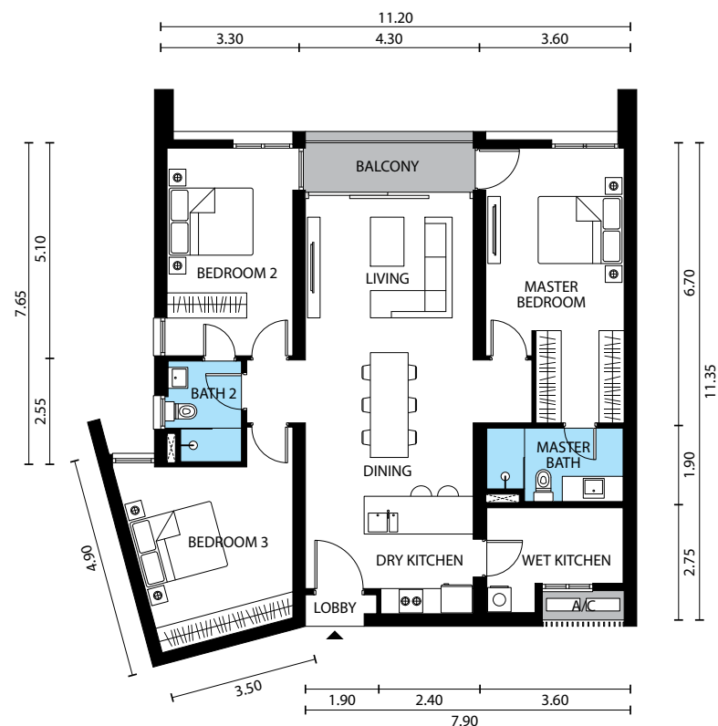
Floor Plan of units in level 5–13a & 21–23a (For others, the dimensions are slightly larger)
