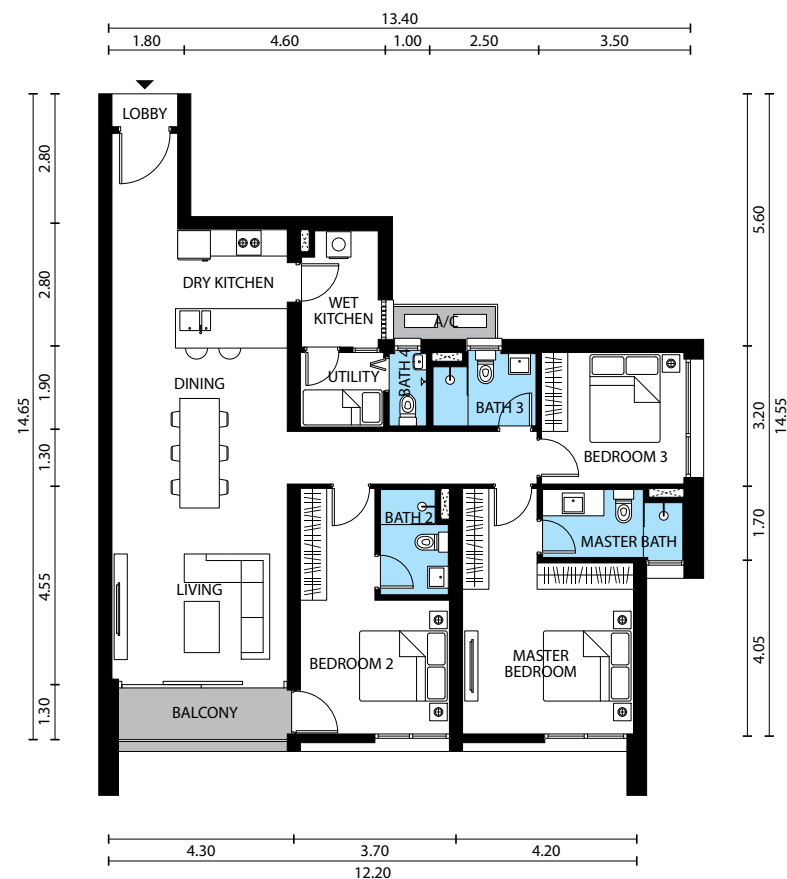
Floor Plan of units in level 11–17 & 23a (For others, the dimensions are slightly larger)
