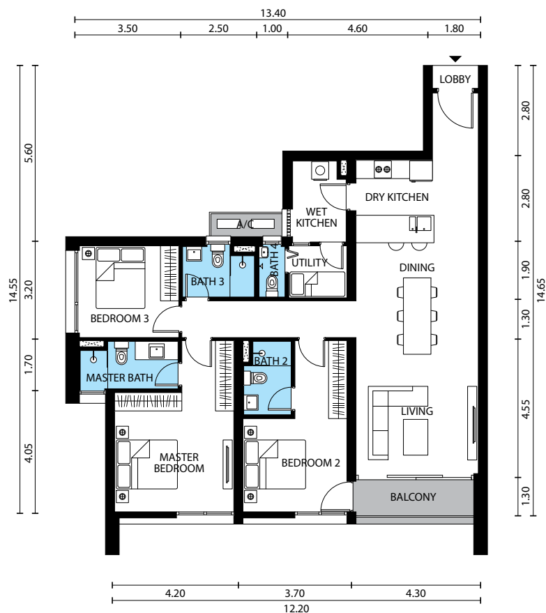
Floor Plan of units in level 7-15 (For others, the dimensions are slightly larger)
