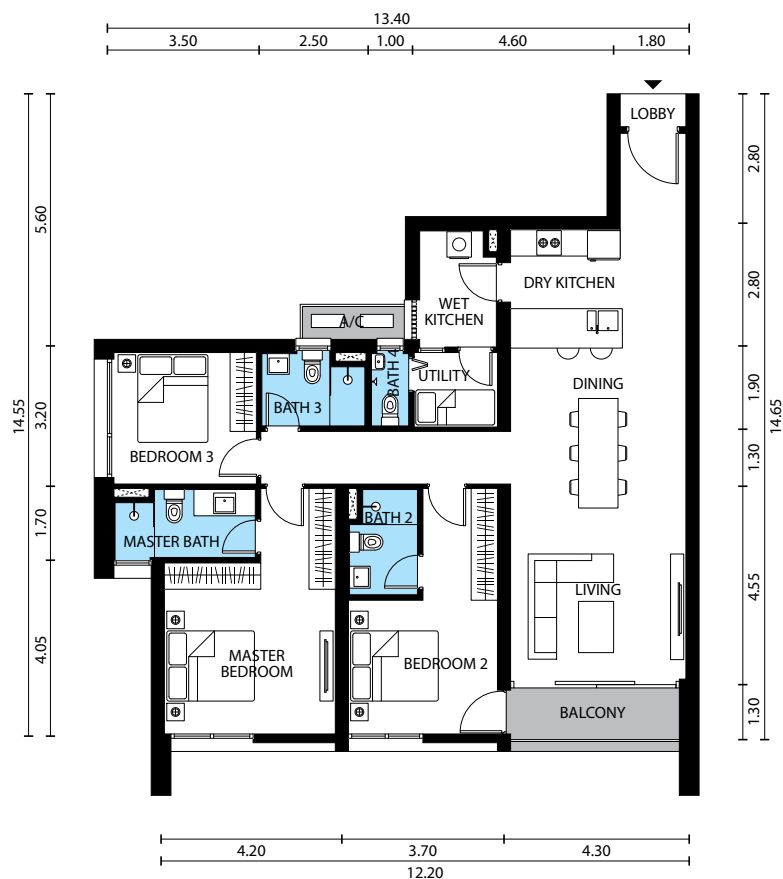
Floor Plan of units in level 18–22 (For others, the dimensions are slightly larger)
