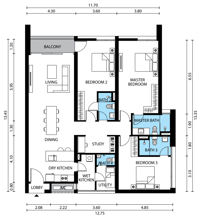
Floor Plan of units in level 9–19 (For others, the dimensions are slightly larger)
