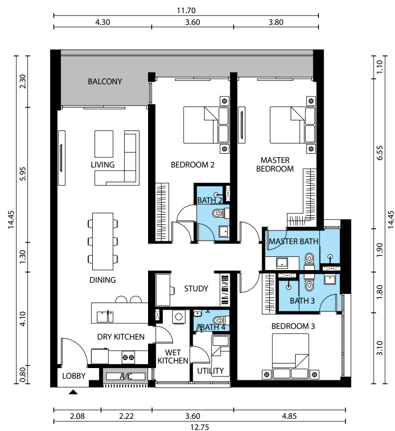
Floor Plan of units in level 3a, 8 & 21 (For others, the dimensions are slightly larger)
