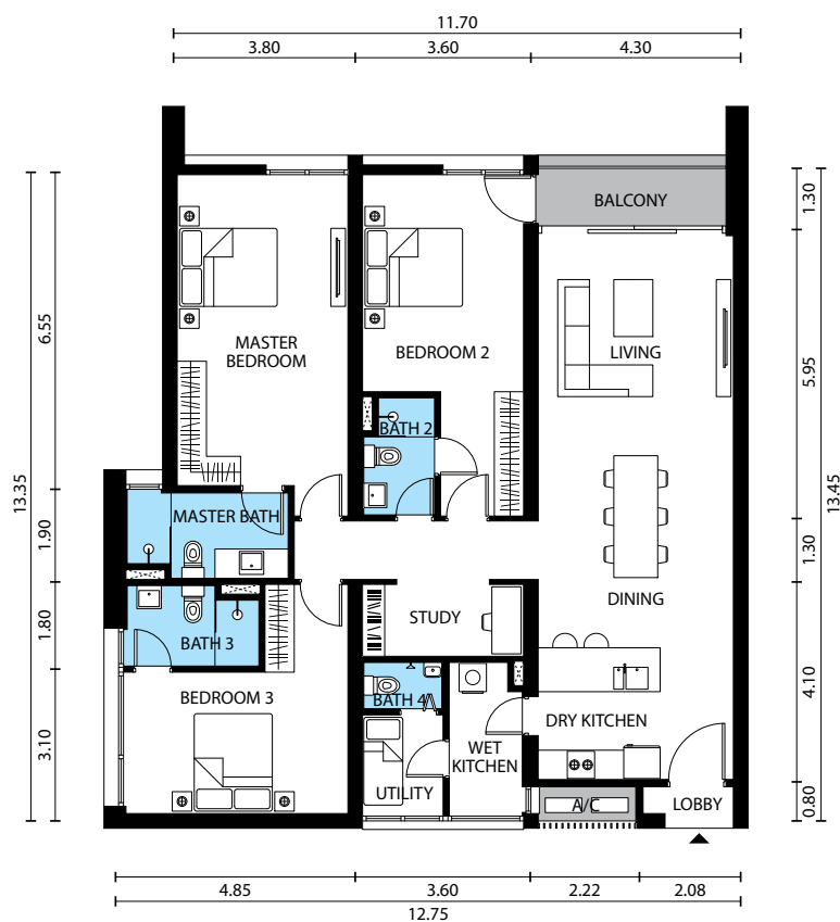
Floor Plan of units in level 5–11 (For others, the dimensions are slightly larger)
